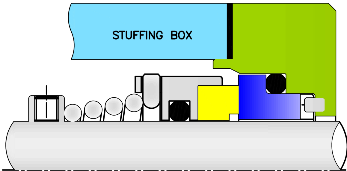
IS-2401 CONICAL SPRING SEAL
