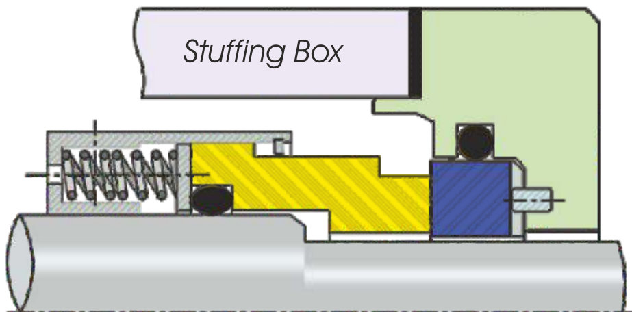
ISPL-2402 Multi Spring Seal Balanced Type
