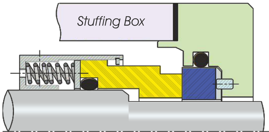
ISPL-2402 Multi Spring Seal Balanced Type
