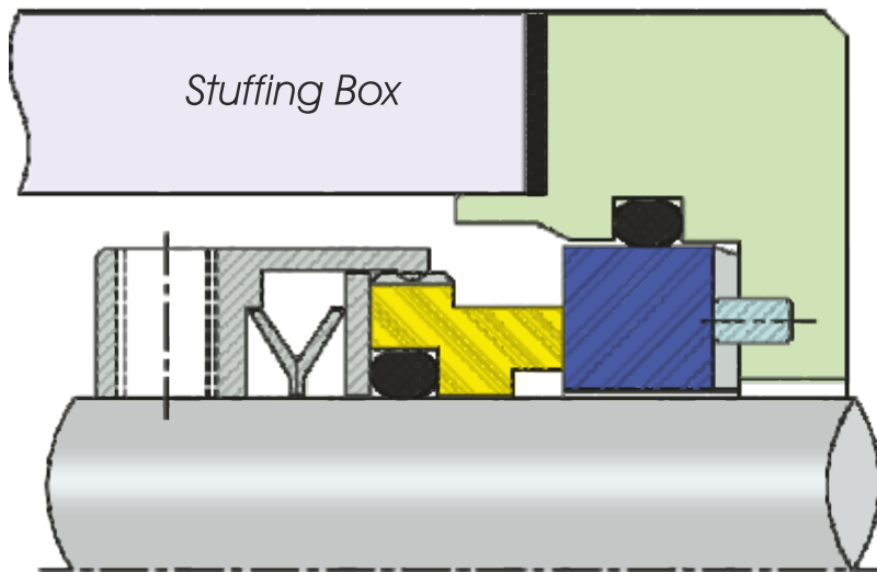
ISPL-2403 Wave Spring UB 'O' Ring Type
