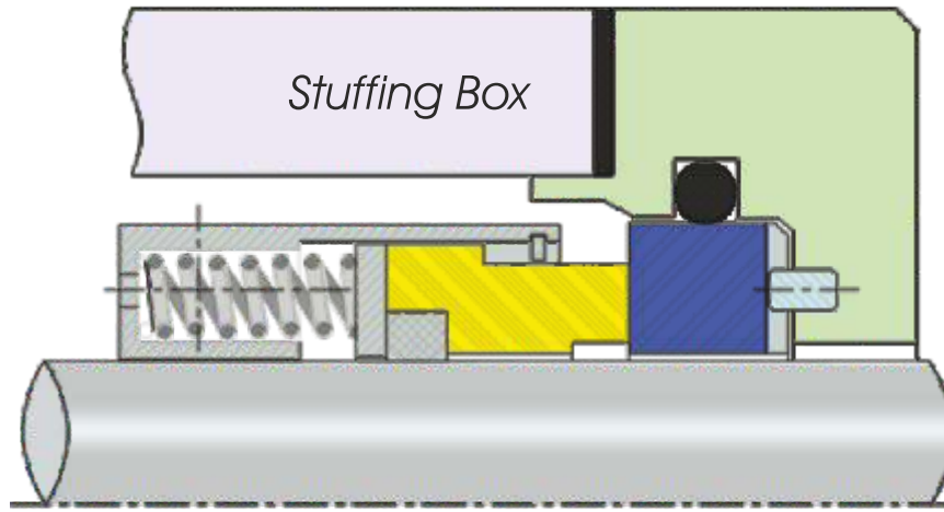
ISPL-2403 Multi Spring Seal UB 'O' Ring Type
