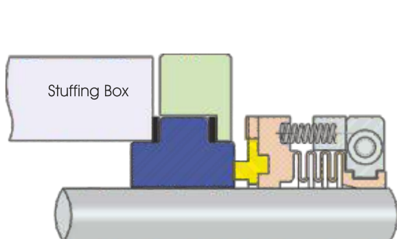
ISPL-2405 Teflon Bellow Multi Spring Seal
