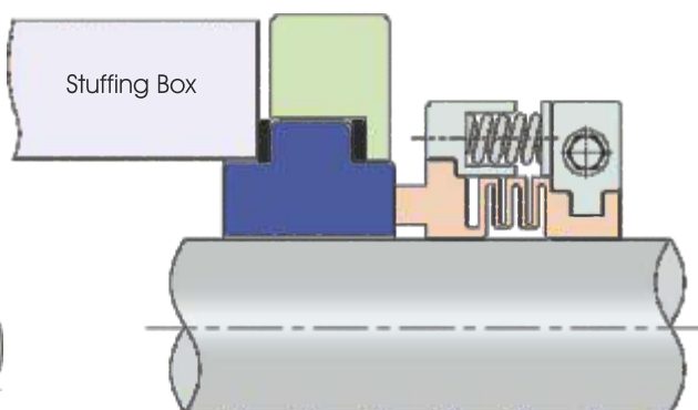
ISPL-2405 Multi Spring with Impregnated Seal Face
