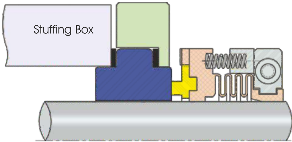
ISPL-2405 Teflon Bellow Multi Spring Seal
