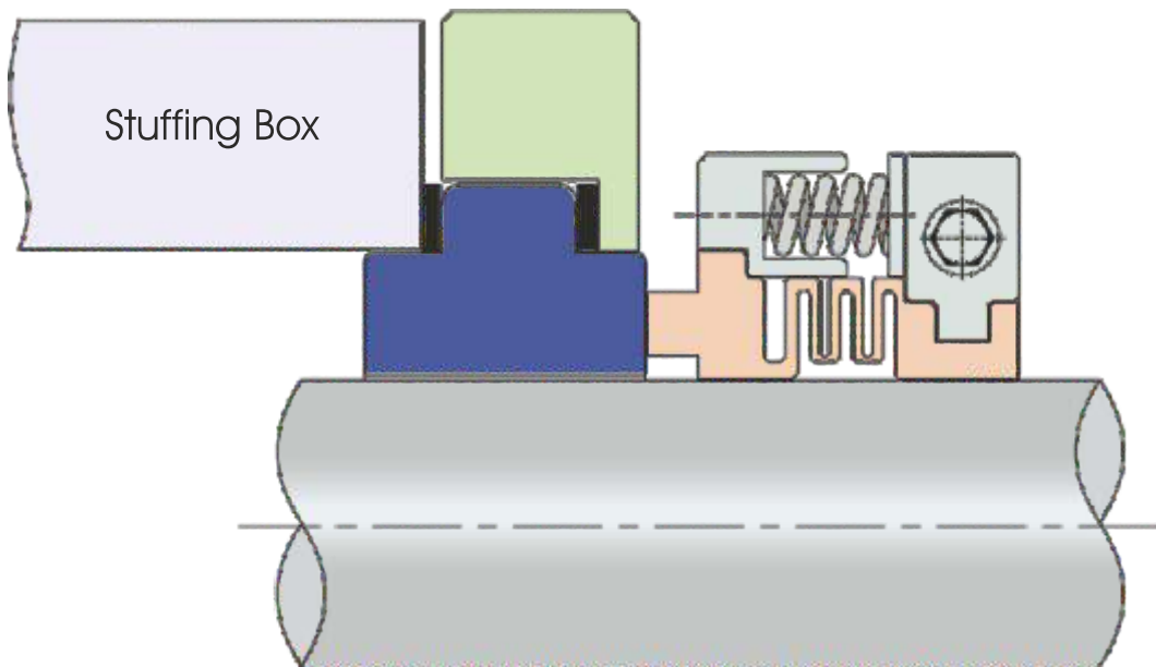
ISPL-2405 Multi Spring with Impregnated Seal Face
