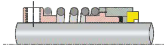
ISPL-2406C Single Spring Special Type Seal
