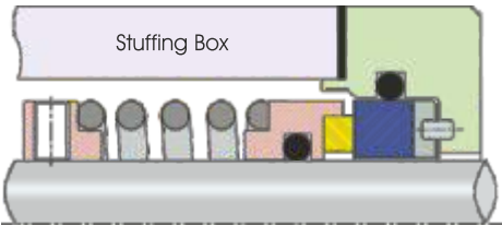
ISPL-2406 Unbalanced Type Seal
