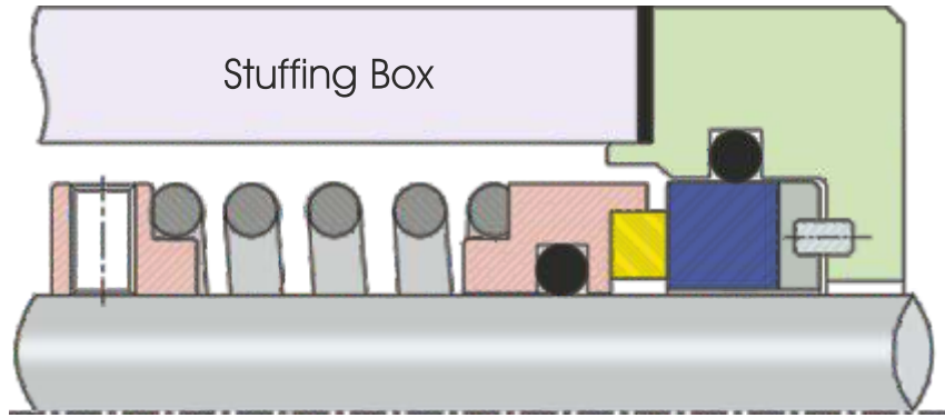
ISPL-2406 Unbalanced Type Seal
