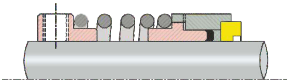
ISPL-2406C Single Spring Special Type Seal
