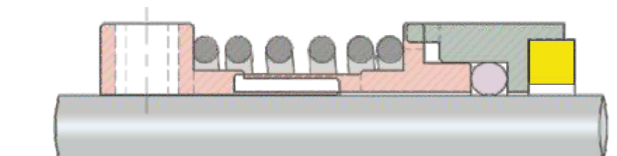
ISPL-2406D Straight Spring Star Type Seal
