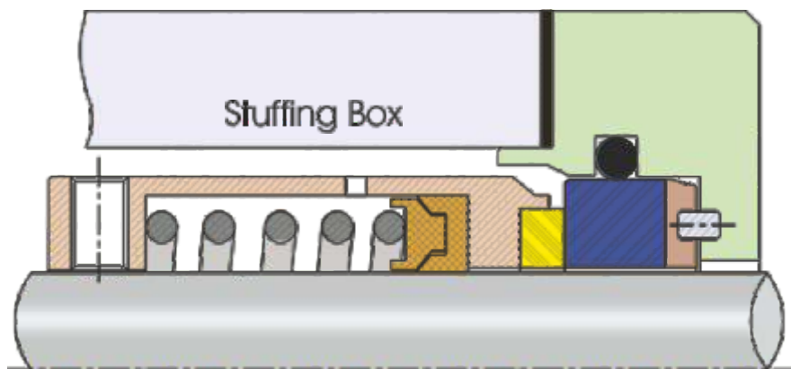
IS-2407 Star Mechanical Seal
