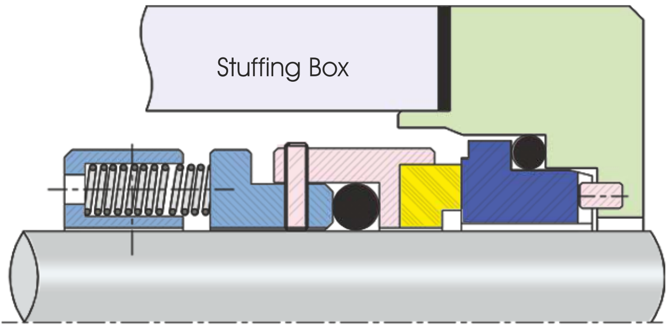
ISPL-2410 Heavy Duty Seal
