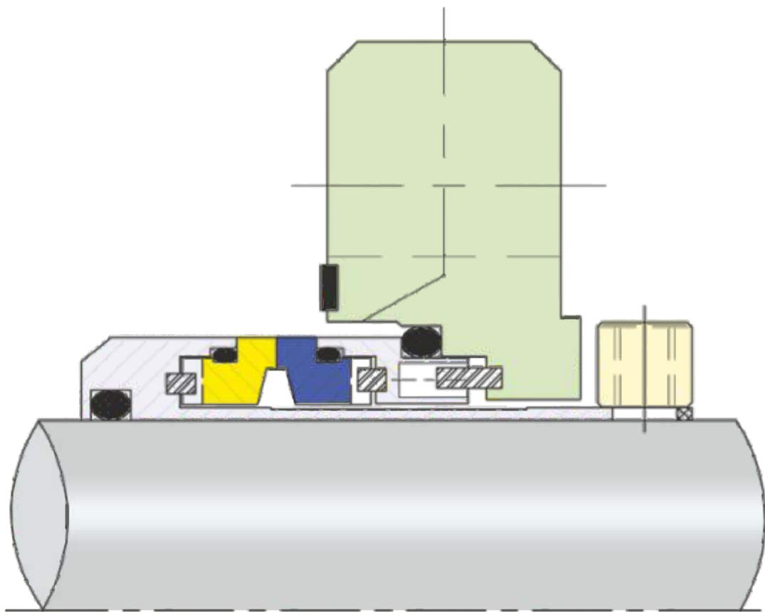
ISPL-2413 Multi Spring Cartridge Type
