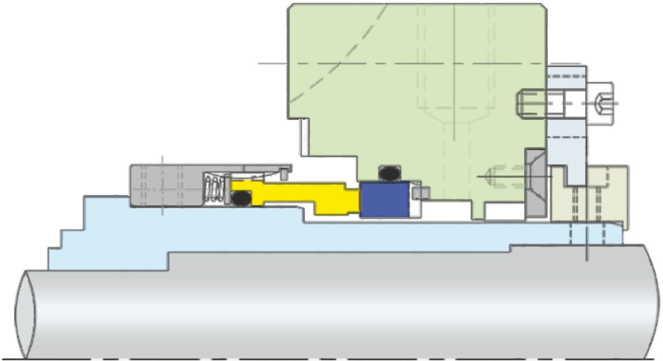
ISPL-2414 Cartridge Seal
