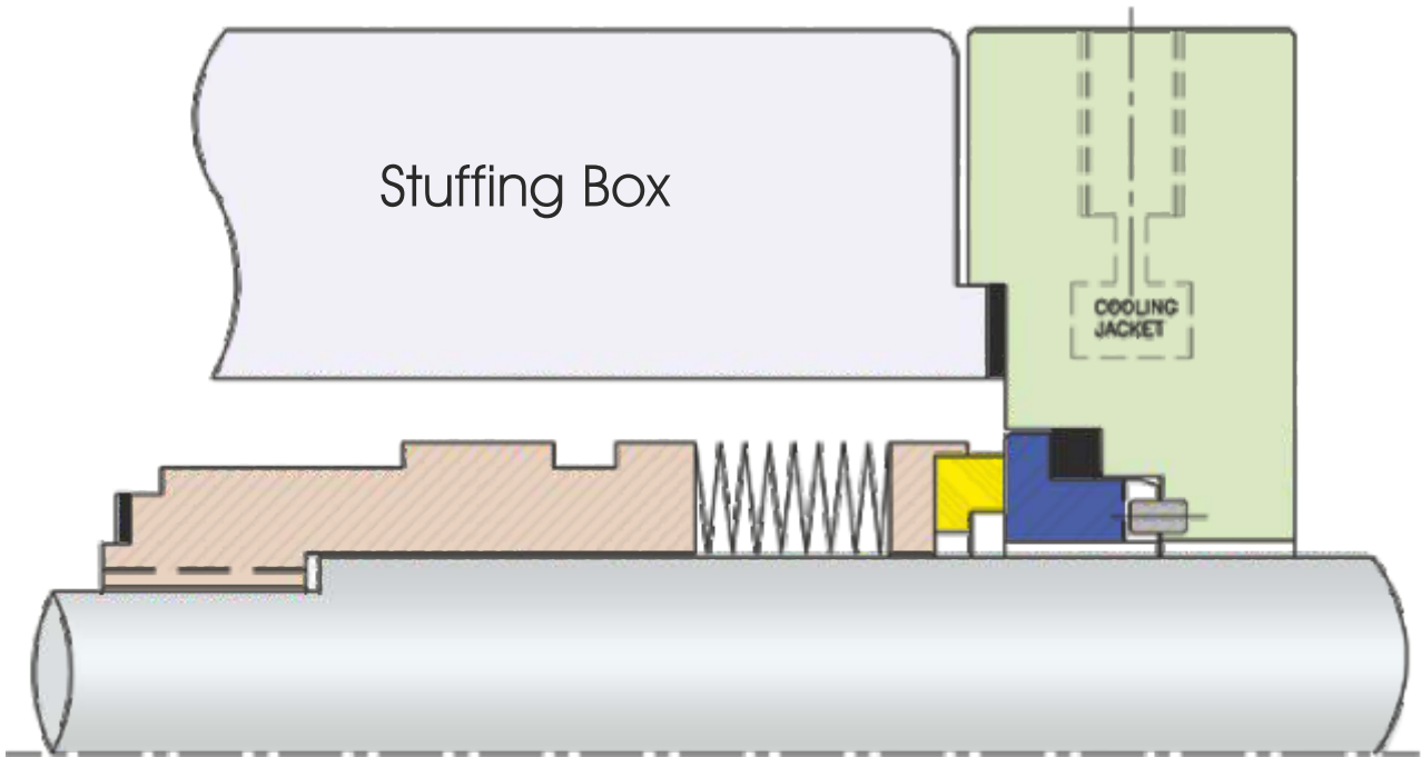
ISPL-2415A Sleeve Welded Bellow Seal
