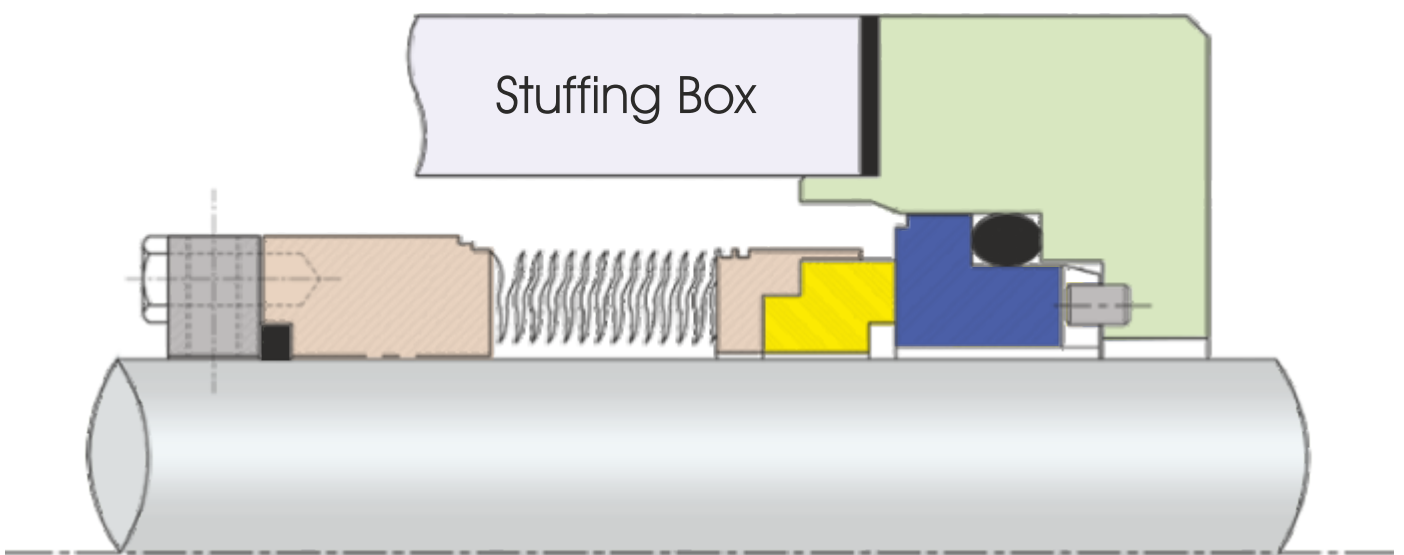
ISPL-2415 Steel Bellow Seal
