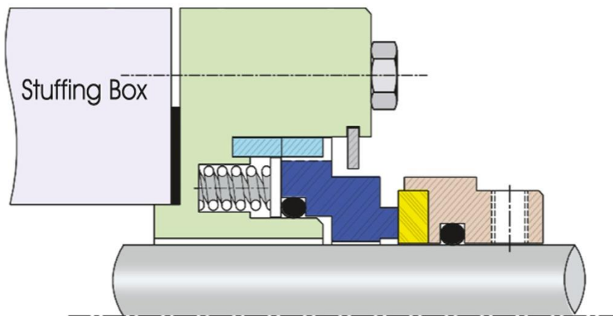
ISPL-2420 Externally Balanced
