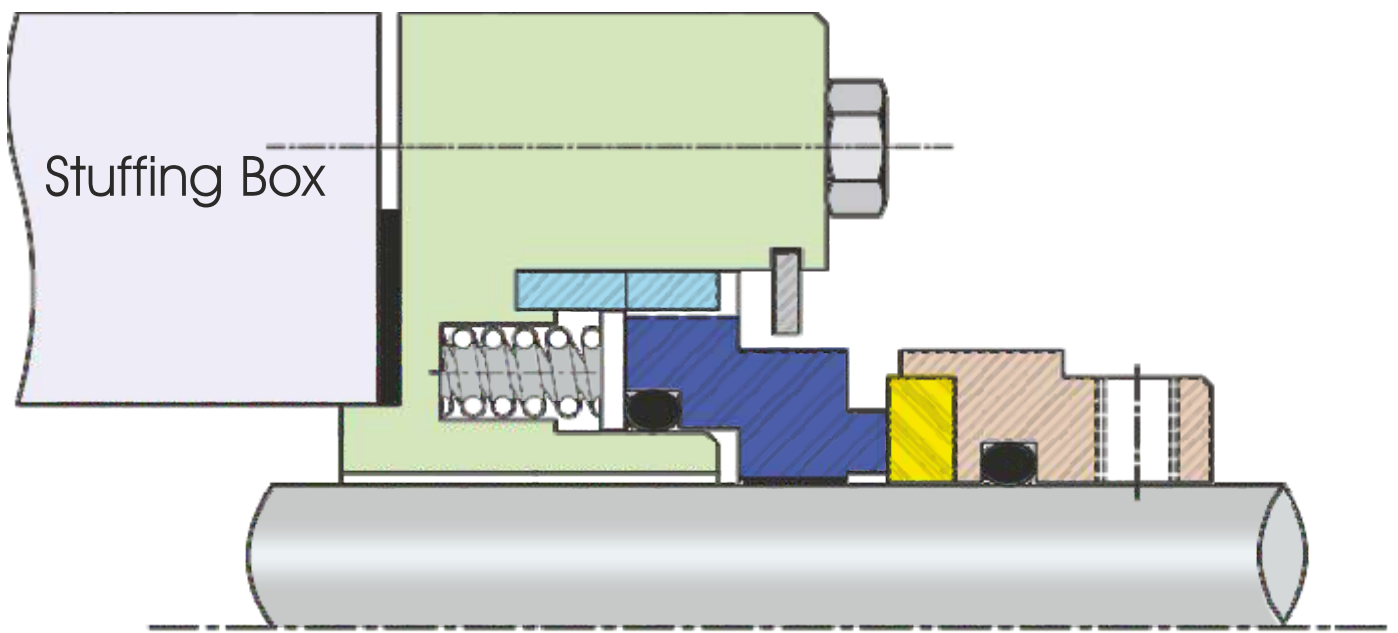
ISPL-2420 Externally Balanced
