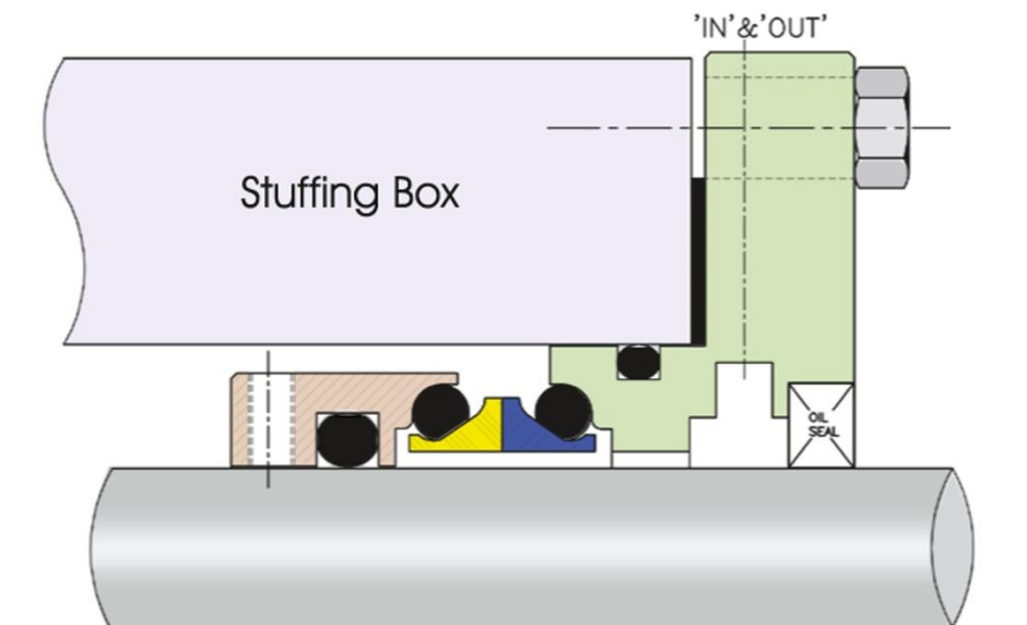
ISPL-2421 Springless Seal
