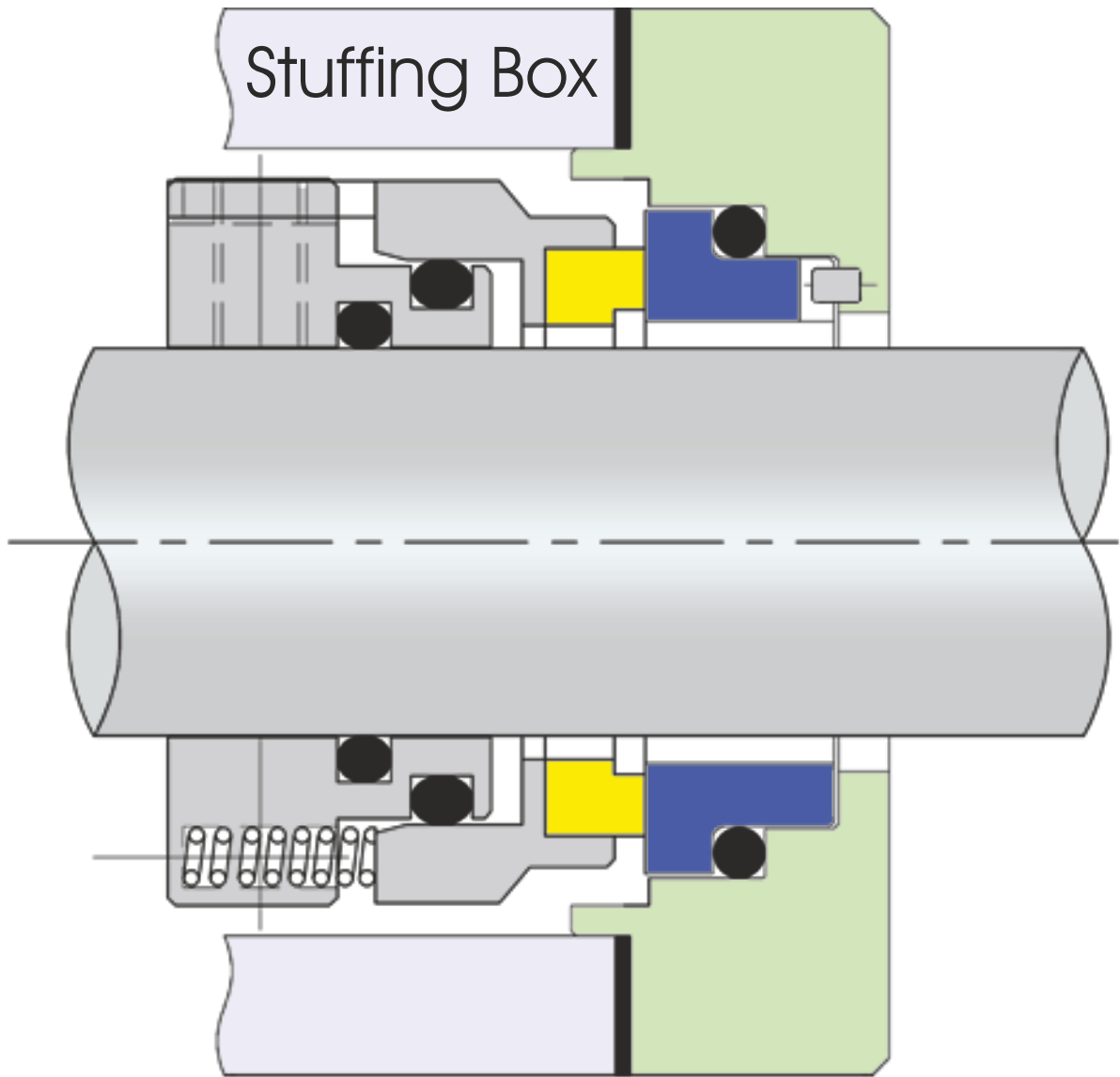
ISPL-2422 RTBS Seal
