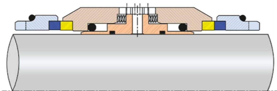
ISPL-2424 DMS for Pressure Screen with Multi Spring
