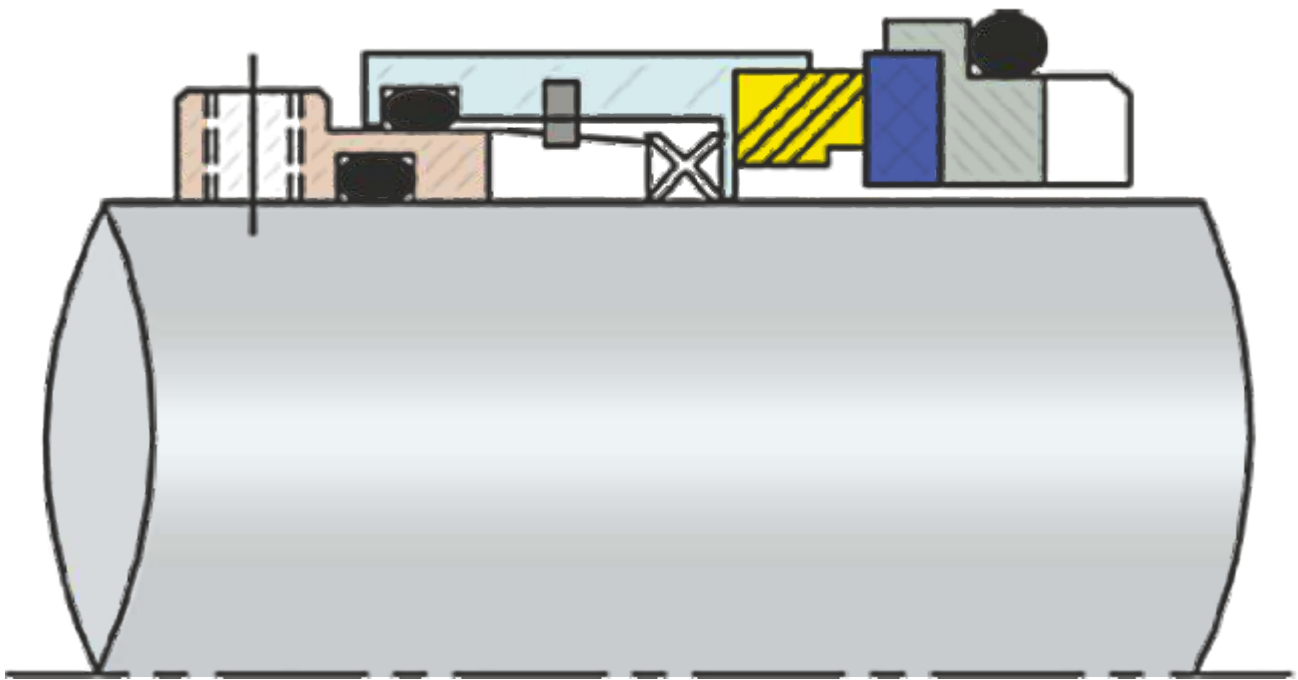
ISPL-2428 Balanced Type Wave Spring Seal
