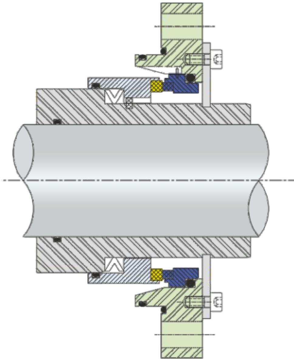
ISPL-2429 Side Entry Agitator Cartridge Type Seal
