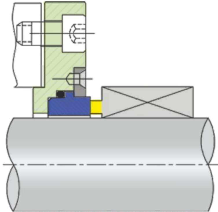
ISPL 24555 Single Seal
