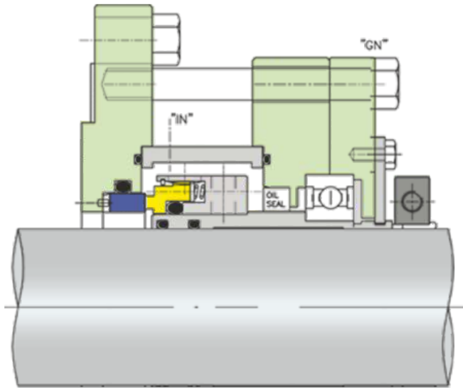
ISPL 24556 Single Seal with Bearing
