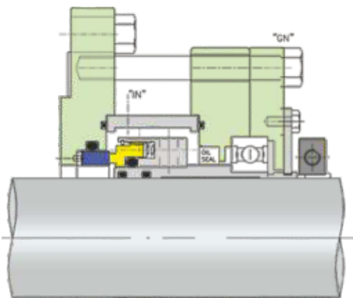
ISPL 24556 Single Seal with Bearing
