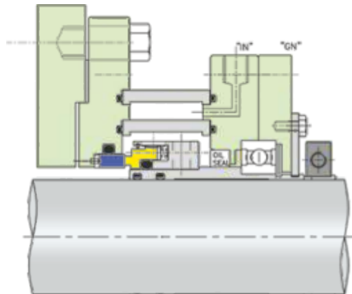
ISPL 24556 A Single Seal with Bearing & Jacketed housing
