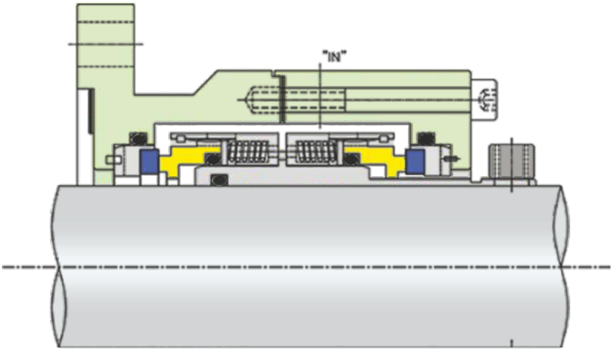
ISPL 24557 A Double Cartridge Balanced type
