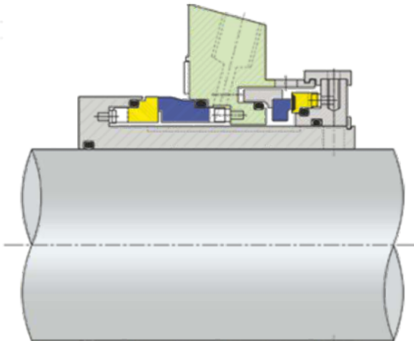
ISPL 24557 B Double Cartridge Mechanical Seal
