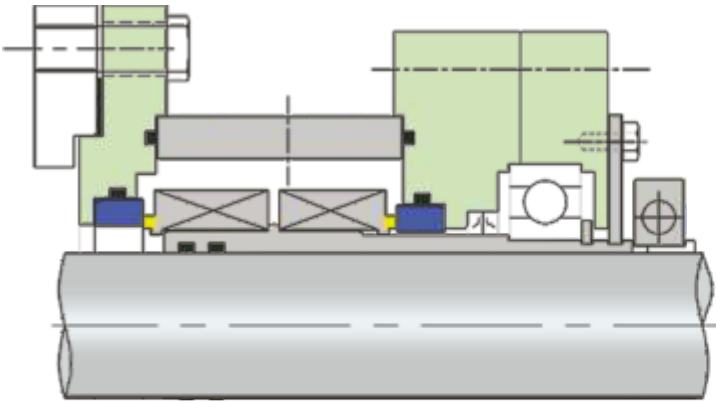
ISPL 24558 Double Cartridge Unbalanced Mechanical Seal with Bearing
