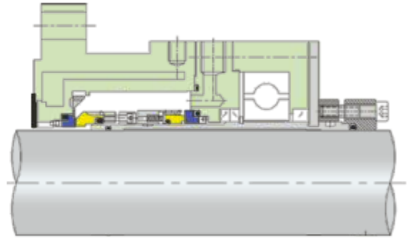
ISPL 24558 A Double Cartridge Balanced Mechanical Seal with Jacketed Housing
