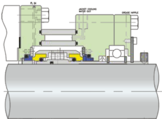
ISPL 24558 B Double Cartridge Common Springs Balanced Mechanical Seal with Sleeve Jacketing
