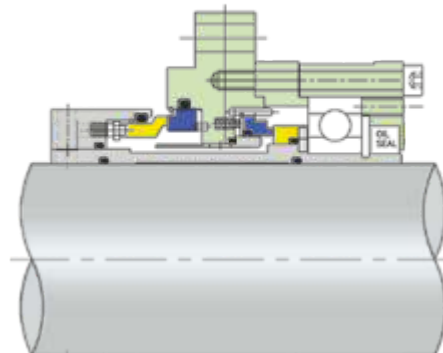
ISPL 24558 E Bottom Entry Double Cartridge Seal with Bearing
