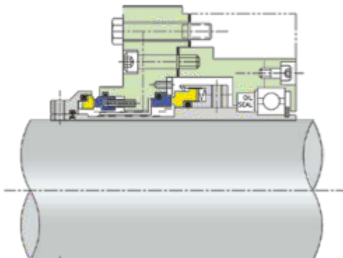
ISPL 24558 D Bottom Entry Double Cartridge Seal with Bearing
