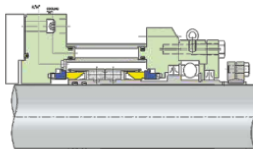
ISPL 24558 C Double Cartridge with Wedge Jacketing Housing, Special Coupling type with bearing
