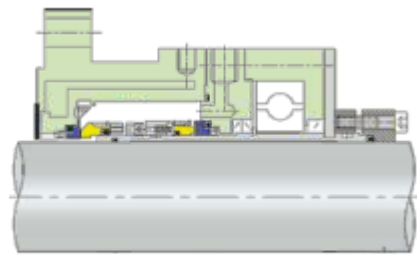
ISPL 24558 A Double Cartridge Balanced Mechanical Seal with Jacketed Housing
