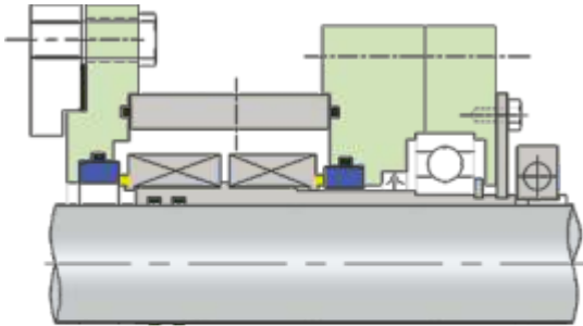
ISPL 24558 Double Cartridge Unbalanced Mechanical Seal with Bearing
