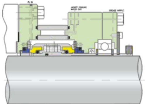
ISPL 24558 B Double Cartridge Common Springs Balanced Mechanical Seal with Sleeve Jacketing
