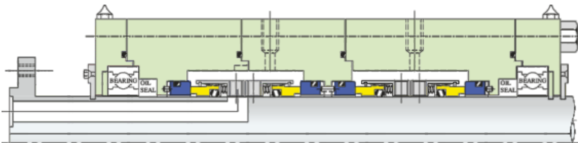
IS-24560 Quadruple Mechanical Seal
