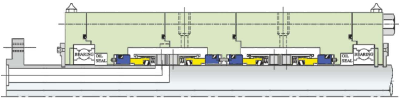
IS-24560 Quadruple Mechanical Seal
