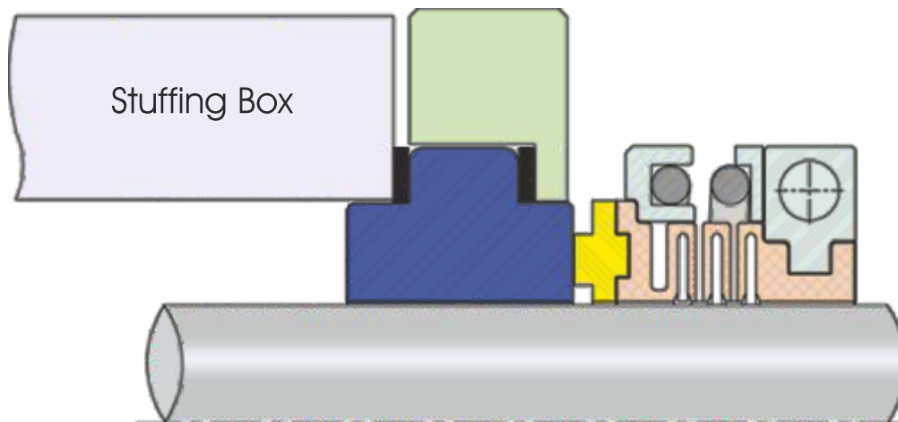
ISPL-2404 Teflon Bellow Single Spring Seal
