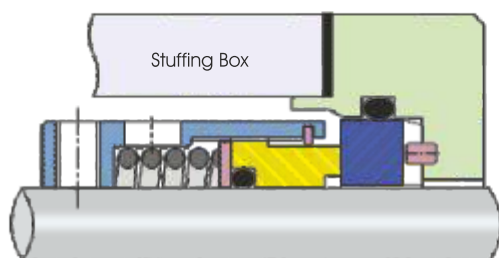
ISPL-2411 Single Spring Cup Type with 'O' ring
