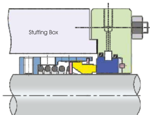
ISPL-2411 With PTFE Wedge Type
