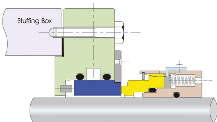
ISPL-2417A Jacketed GP Type
