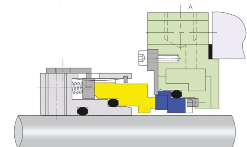
ISPL-2417B Jacketed plate Type
