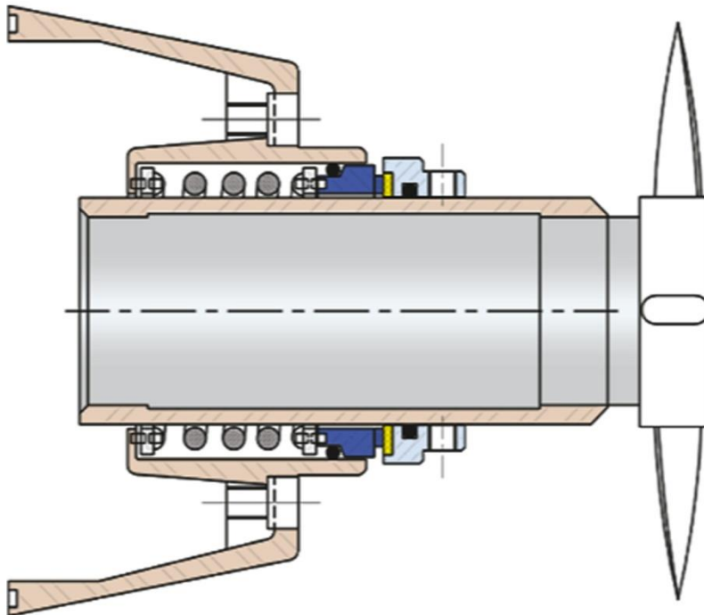
ISPL-2425 Single Spring Seal
